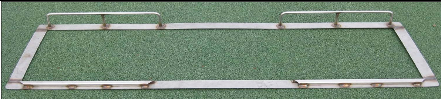
B Front view of front rail. 1/4 inch box steel tubing. This tubing is in front of front wheelchair wheels to keep chair from rolling forward during swing, but small enough to easily push over after hit and when accelerating wheelchair.
